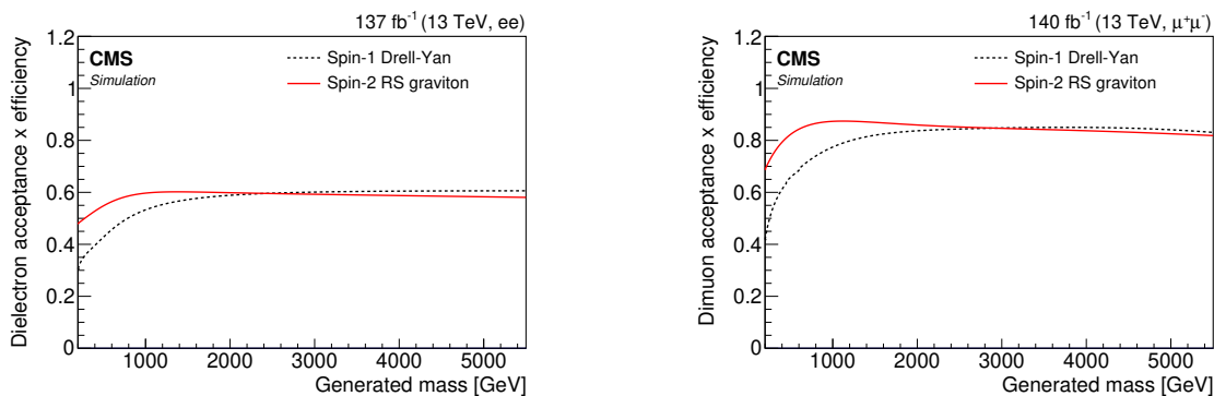
Figure 1. Product of the acceptance and the efficiency for (left) dielectron and (right) dimuon pairs as a function of generated mass in simulated events. The DY samples are used to represent spin-1 particles, and RS graviton samples are used for spin-2 particles.
