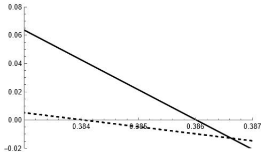
Figure 3. Graph of T_2 \cdot \frac{24a^2(a^2+1)}{k^2} (dashed line) and T_3 \cdot \frac{72a^2(a^2+1)^2}{k^3} (solid line) near a_* \approx 0.384479856571409680884645 .
