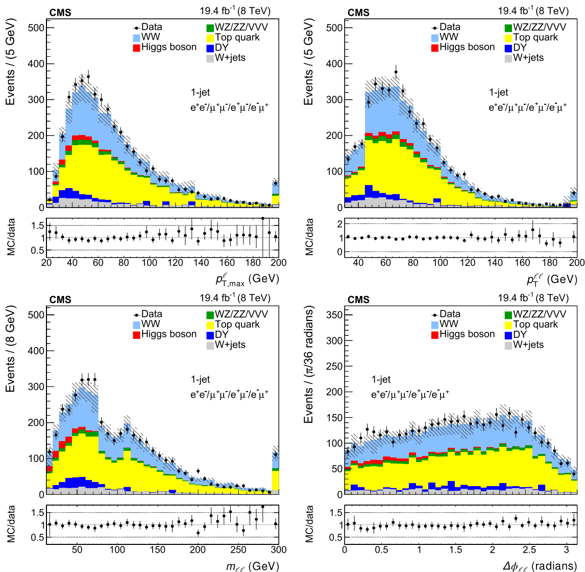
Fig. 2 The data and MC distributions for the one-jet category of the leading lepton p_T ( p_{T,max}^l ), the p_T of the dilepton system ( p_T^{ll} ), the dilepton invariant mass ( m_{\ell\ell} ) and the azimuthal angle between the two leptons ( \Delta\phi_{\ell\ell} ). The hatched areas represent the total systematic uncer-
