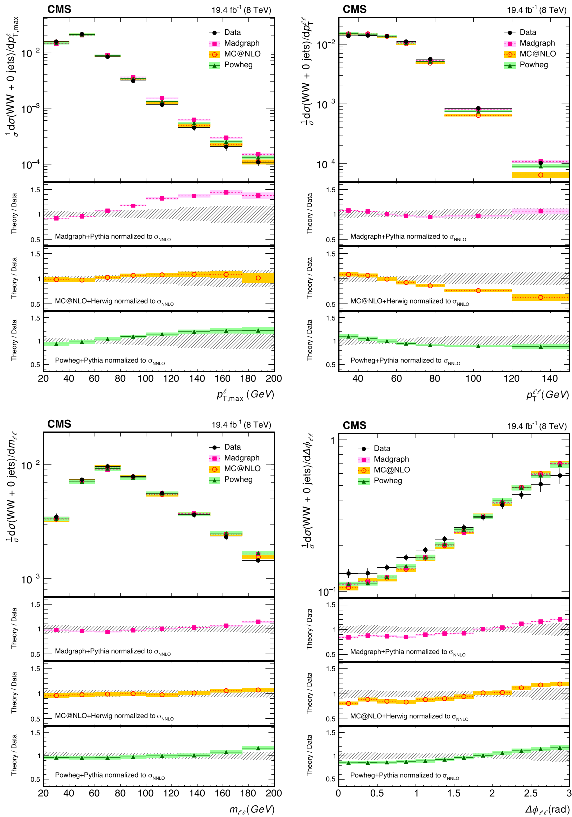
Fig. 3 Normalized differential W^+W^- cross section as a function of the leading lepton p_T ( p_{T, \max}^{\ell} ) (top left), the transverse momentum of the dilepton system ( p_T^{\ell\ell} ) (top right), the invariant mass ( m_{\ell\ell} ) (bottom left) and the angular separation between leptons ( \Delta\phi_{\ell\ell} ) (bottom right).
