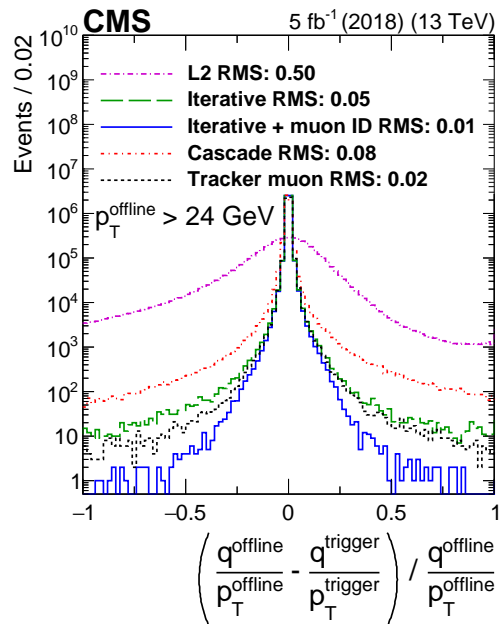
Figure 7. The q/p_T residual distributions integrated over \eta and p_T for all different HLT muon reconstruction algorithms used in 2018. Only statistical uncertainties are shown.
