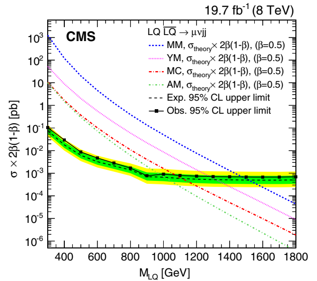
FIG. 14. Frame on top (bottom): the expected and observed upper limits at 95% CL on the vector leptoquark pair production cross section times \beta^2 ( 2\beta(1-\beta) ) as a function of the second generation vector leptoquark mass, obtained with the \mu\mu jj ( \mu\nu jj ) analysis for the four coupling scenarios (MC, YM, MM, and AM). The expected limits and uncertainty bands represent the median expected limits and the 68% and 95% confidence intervals using the MC scenario. Because of the kinematic similarity between the MC scenario and the other coupling scenarios, cross section limits are found to be the same within the uncertainties.
