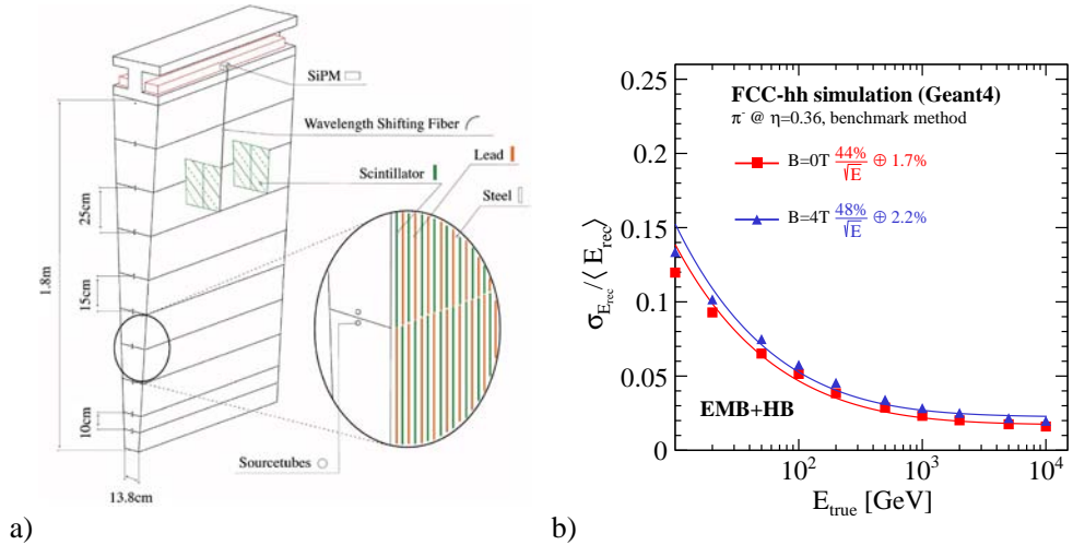
Fig. 7.18. (a) Barrel HCAL technology based on scintillators similar to the ATLAS TileCal. (b) Combined single pion resolution of the barrel EMB + HB using a benchmark hadronic calibration method [357].
