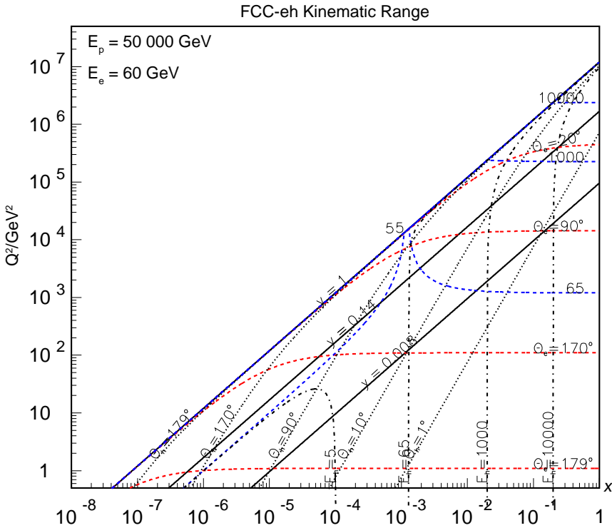
Fig. 7.27. Kinematics of the FCC-eh for E_p = 50 \text{ TeV} and E_e = 60 \text{ GeV} . Blue dashed lines: constant scattered electron energy, which for Q^2 below 1000 \text{ GeV}^2 never exceeds 65 \text{ GeV} . Red dashed lines: constant electron polar angle. One observes that the low x region is very accessible with a detector acceptance down to one degree for backward electrons. Black dashed-dotted lines: constant hadronic final state energy. At large Bjorken x , energies of up to tens of TeV are scattered in the forward detector region; black dotted lines: constant polar angle of the hadronic final state.
