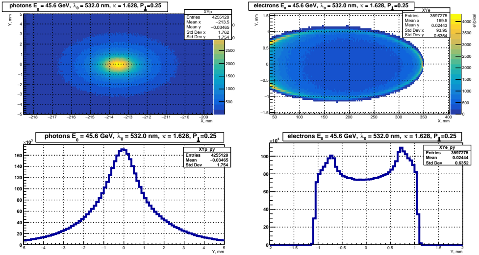
Fig. 3.29. MC results for P_{\perp} = \xi_{\odot} \zeta_{\perp} = 0.25 and \phi_{\perp} = \pi/2 .
