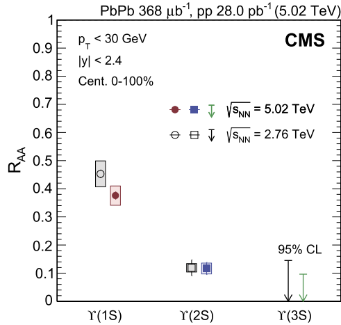
Fig. 7. Comparison of R_{AA} values for the \Upsilon(1S) , \Upsilon(2S) and \Upsilon(3S) mesons at \sqrt{s_{\text{NN}}} = 5.02 \text{ TeV} and \sqrt{s_{\text{NN}}} = 2.76 \text{ TeV} [21] for integrated centrality in the full kinematic range. The error bars represent the statistical uncertainties and the boxes the systematic uncertainties, including global uncertainties.
