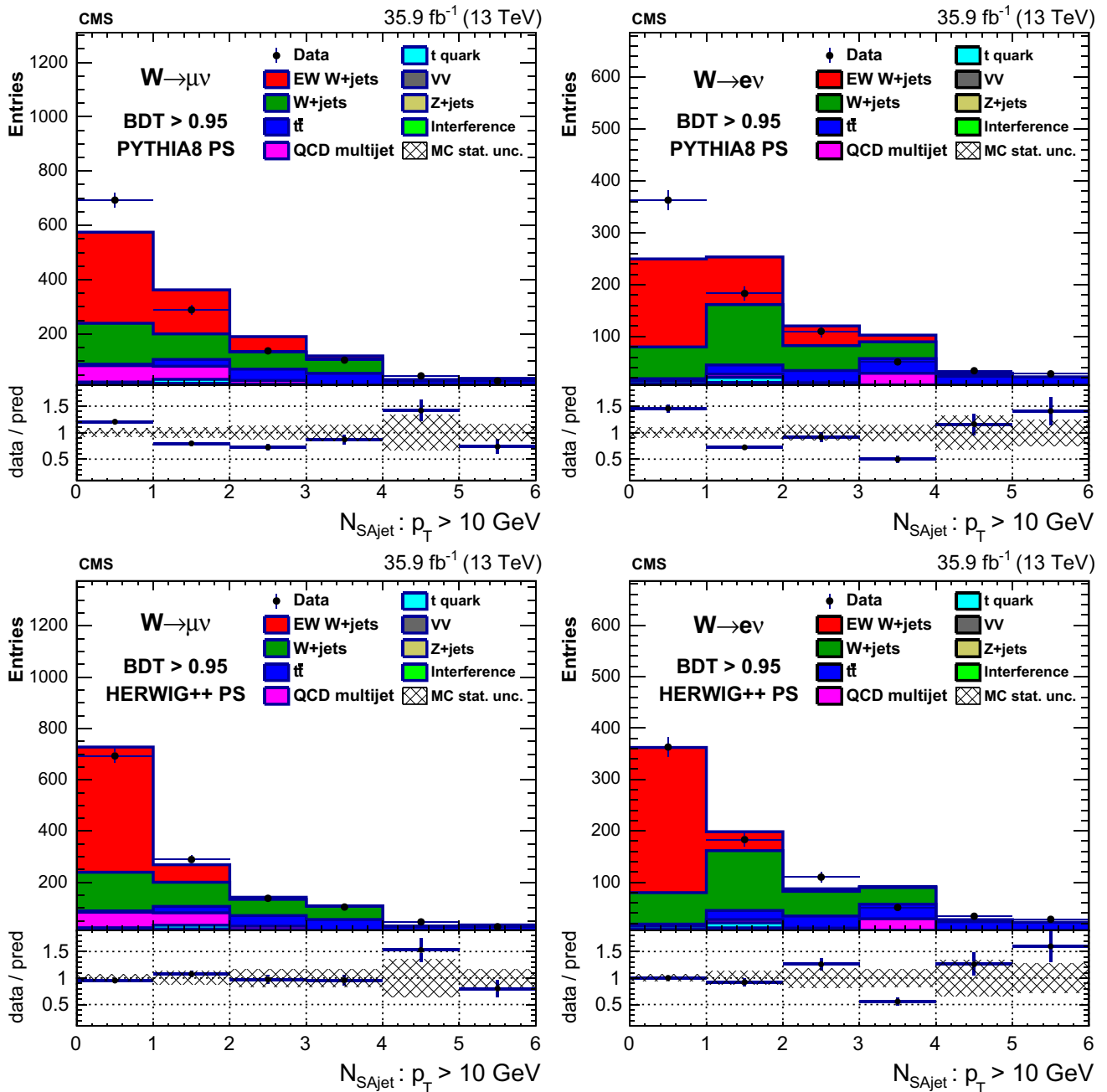
Fig. 20 Number of soft activity jets with p_T > 10 \text{ GeV} in the rapidity gap for \text{BDT} > 0.95 in the muon (left) and electron (right) channels including signal with PYTHIA parton showering (upper) and HERWIG++ parton showering (lower). In all plots the last bin contains overflow events
